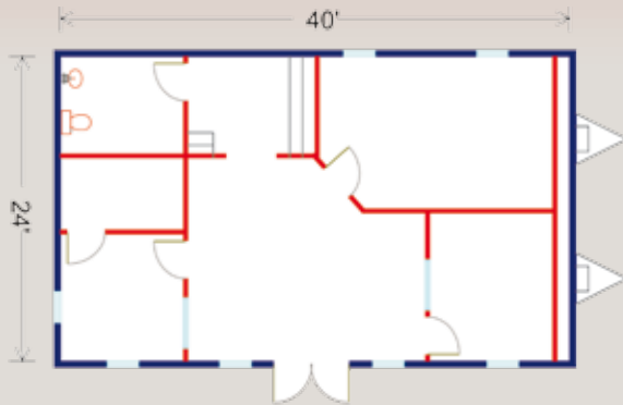
Model 2440S
