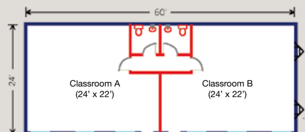
Model 2460C (Plan B)
