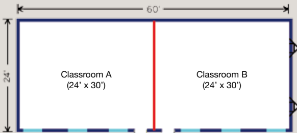
Model 2460C (Plan A)
